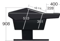
V Series profile with V1000 rack module.
