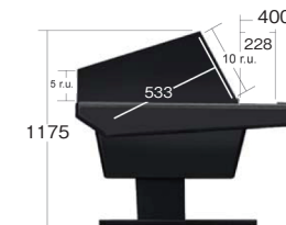
V Series profile with V1005 rack module.
