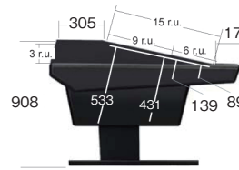
V Series profile with V1503 rack module.
