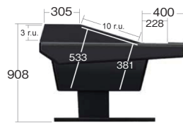
V Series profile with V1003 rack module.
