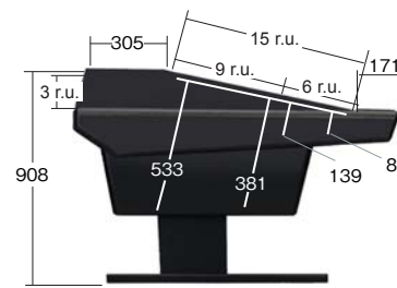
V Series profile with V1503 rack module.
